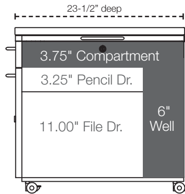
Metal side bin sold separately
