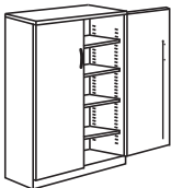
5-high, 4 shelf 65-7/8"
